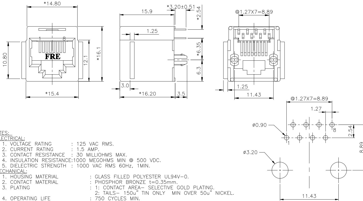
PC Board Layout Component Side Shown
